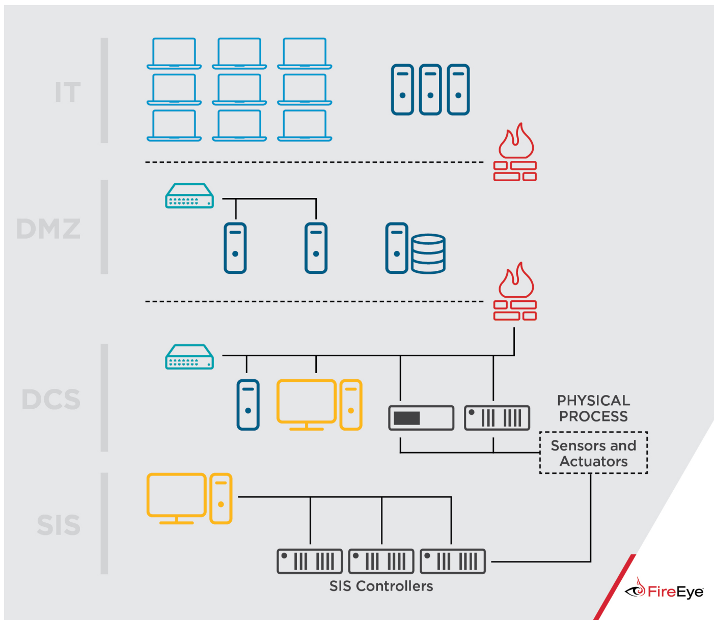
Figure 1: ICS Reference Architecture
